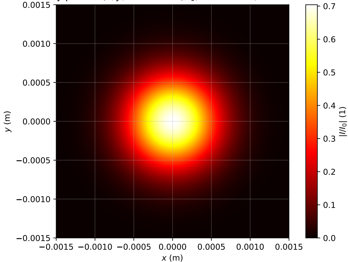
Intensity profile I(x, y, z = 1.433m)/I_0 , Pin=0.1Pcr, artificial time
